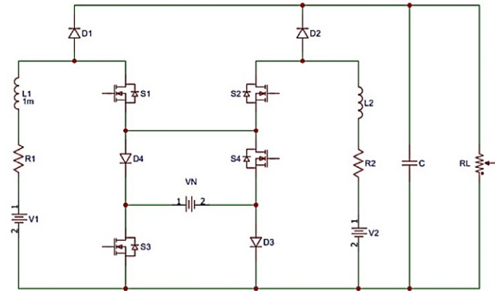
Fig. 1. The proposed schematic diagram for energy supply system
