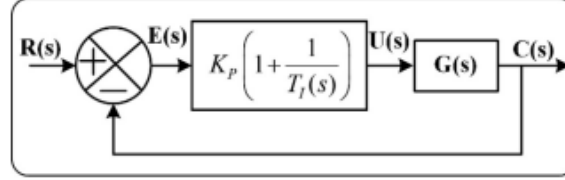
Fig. 3. PI controller block diagram
