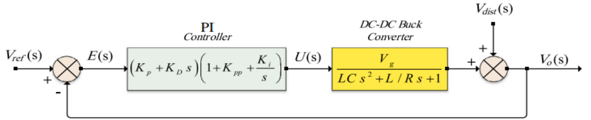
Figure 4. proposed controller diagram
