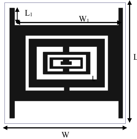
Figure 1. Geometry of the MTM unit cell.
