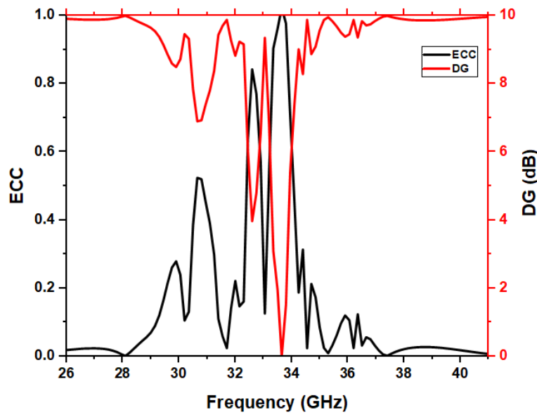
Figure 11. ECC and DG of the MIMO antenna.
