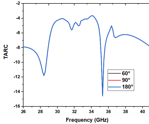
Figure 14. TARC of the MIMO antenna.
